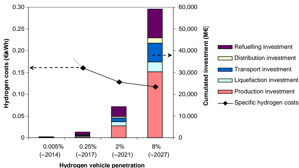
Figure 3.3 Aggregated total hydrogen costs (base case scenario with country-specific feedstock bounds and 20% LH 2 demand at pump of filling station)
