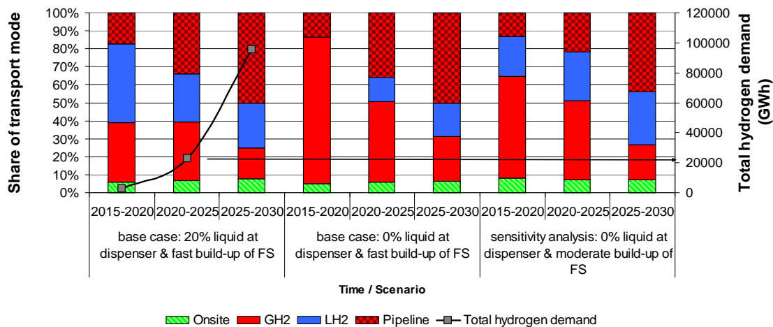
Figure 3.4 Hydrogen transport modes
