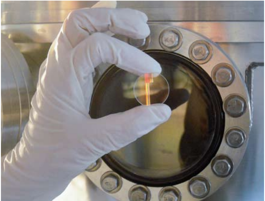
Fig. 4.6.1 Spatially variable transmission filter manufactured by radiofrequency sputtering © ENEA
